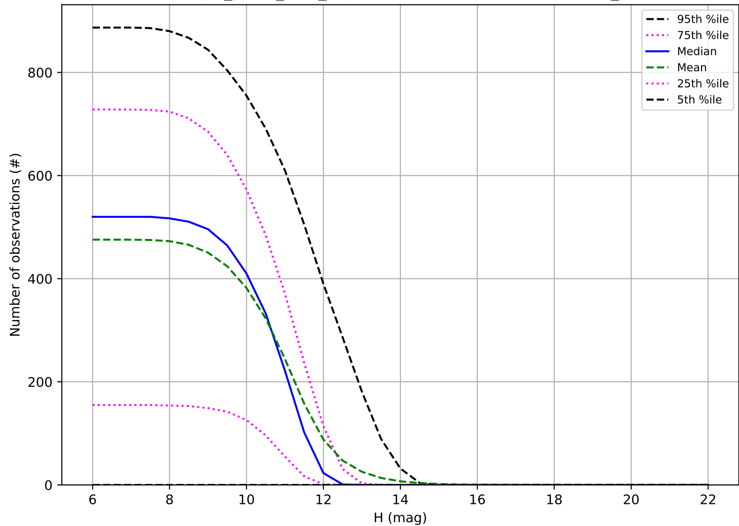
reweight_plane_v3.3_10yrs: Number of observations OCC_r20
