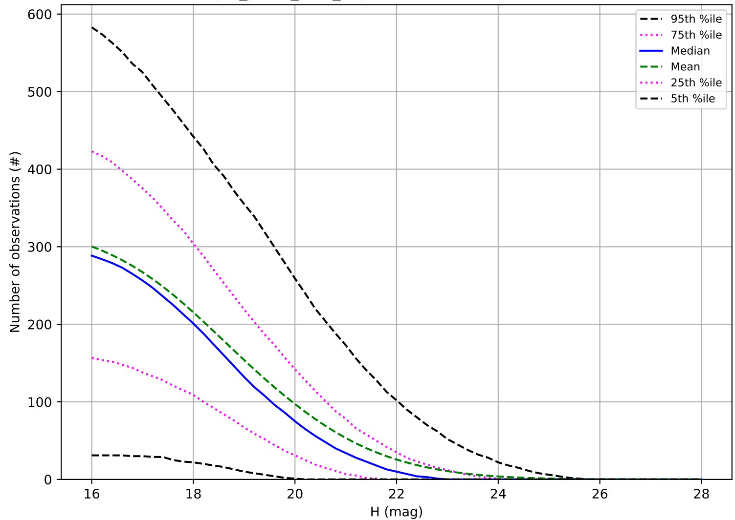
reweight_plane_v3.3_10yrs: Number of observations NEO
