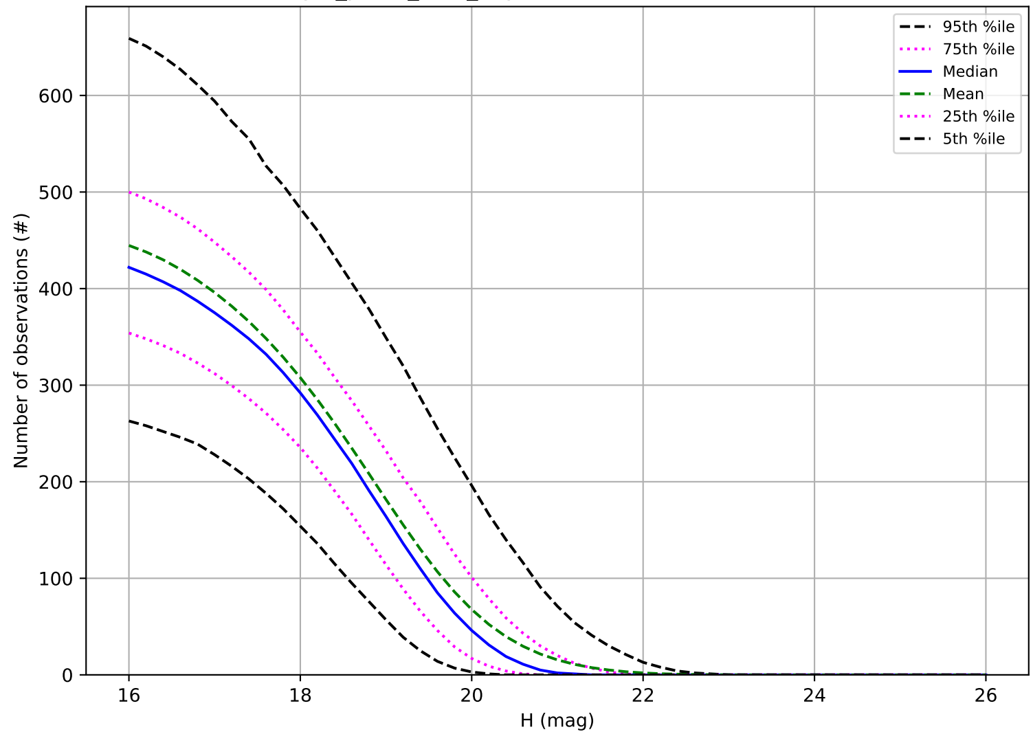
reweight_plane_v3.3_10yrs: Number of observations MBA
