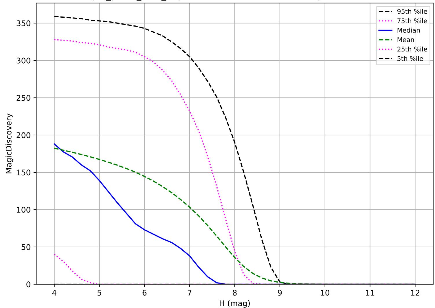
reweight_plane_v3.3_10yrs: TNO 6 detections in 60 nights detection loss
