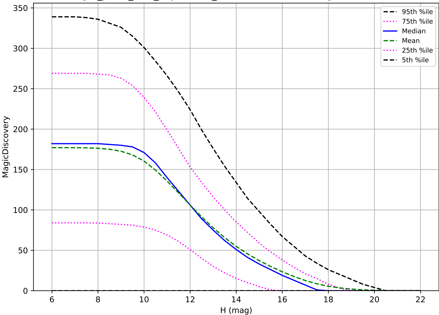
reweight_plane_v3.3_10yrs: OCC_r5 6 detections in 60 nights detection loss
