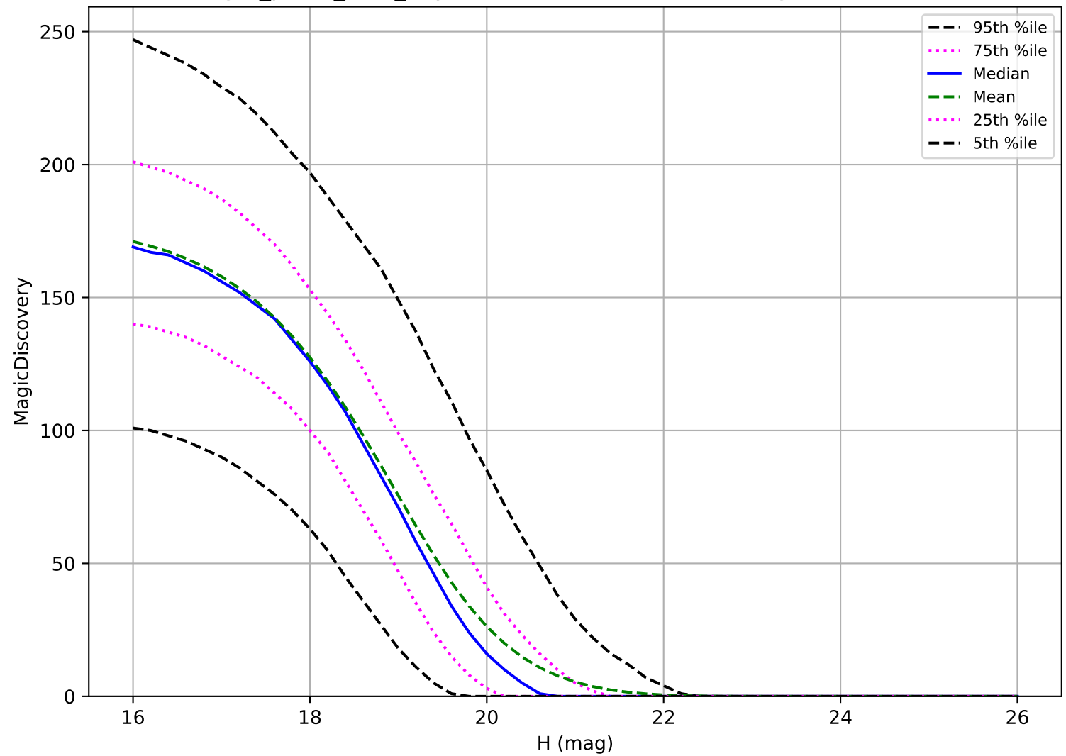
reweight_plane_v3.3_10yrs: MBA 6 detections in 60 nights detection loss
