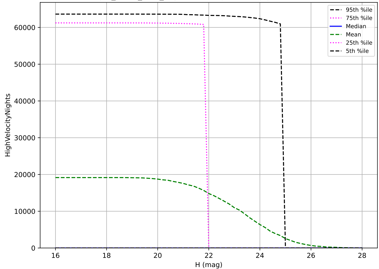
reweight_plane_v3.3_10yrs: NEO High velocity pair detection loss
