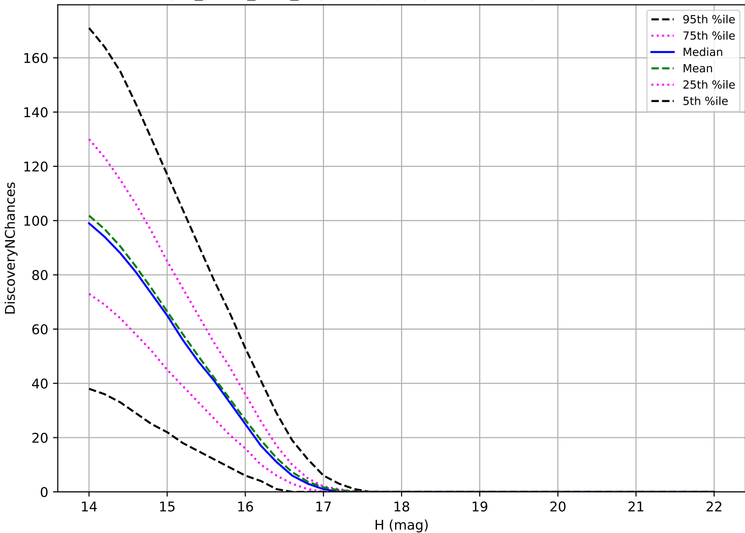
reweight_plane_v3.3_10yrs: Trojan 3 pairs in 15 nights detection loss
