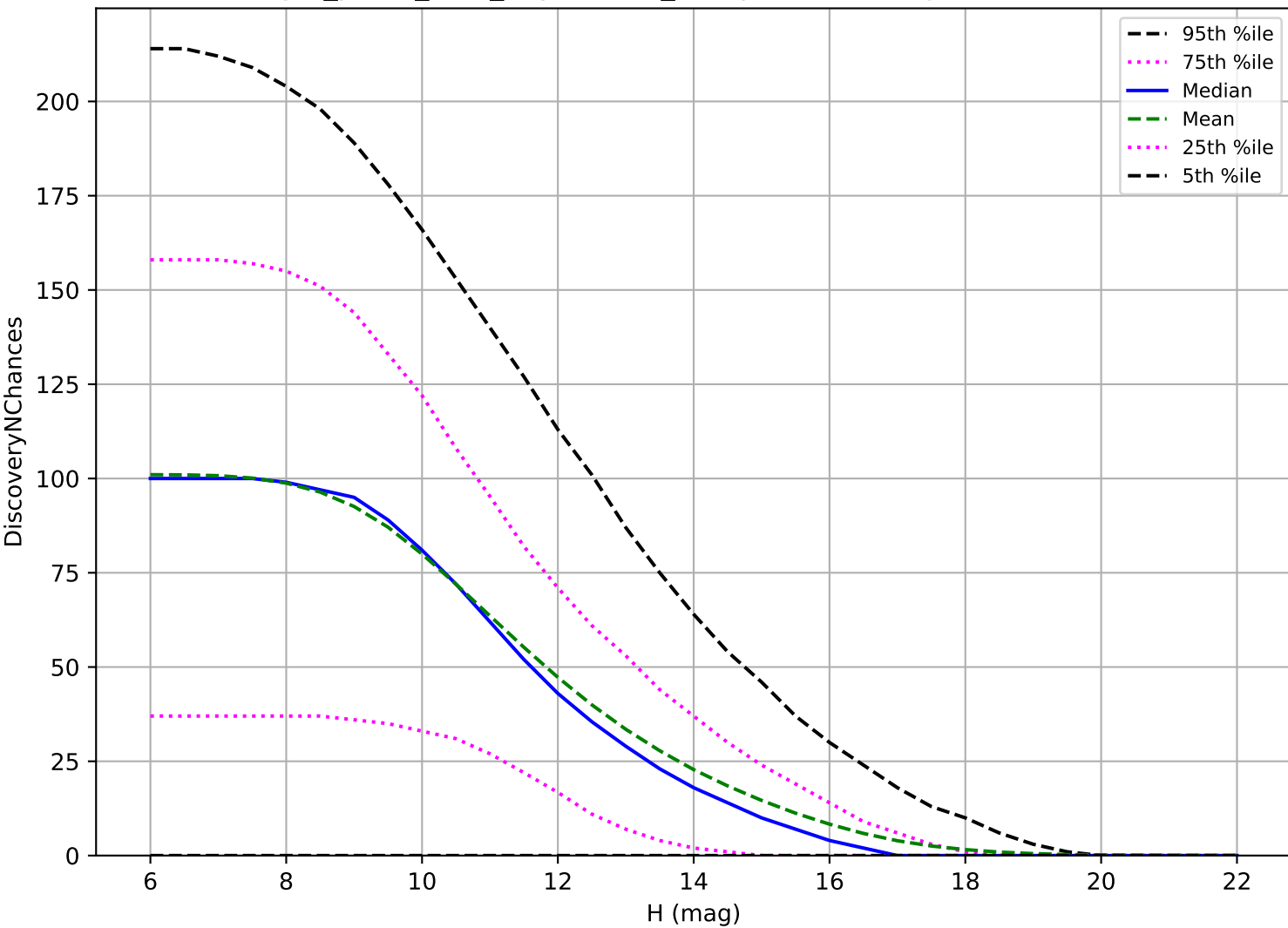
reweight_plane_v3.3_10yrs: OCC_r5 3 pairs in 15 nights detection loss
