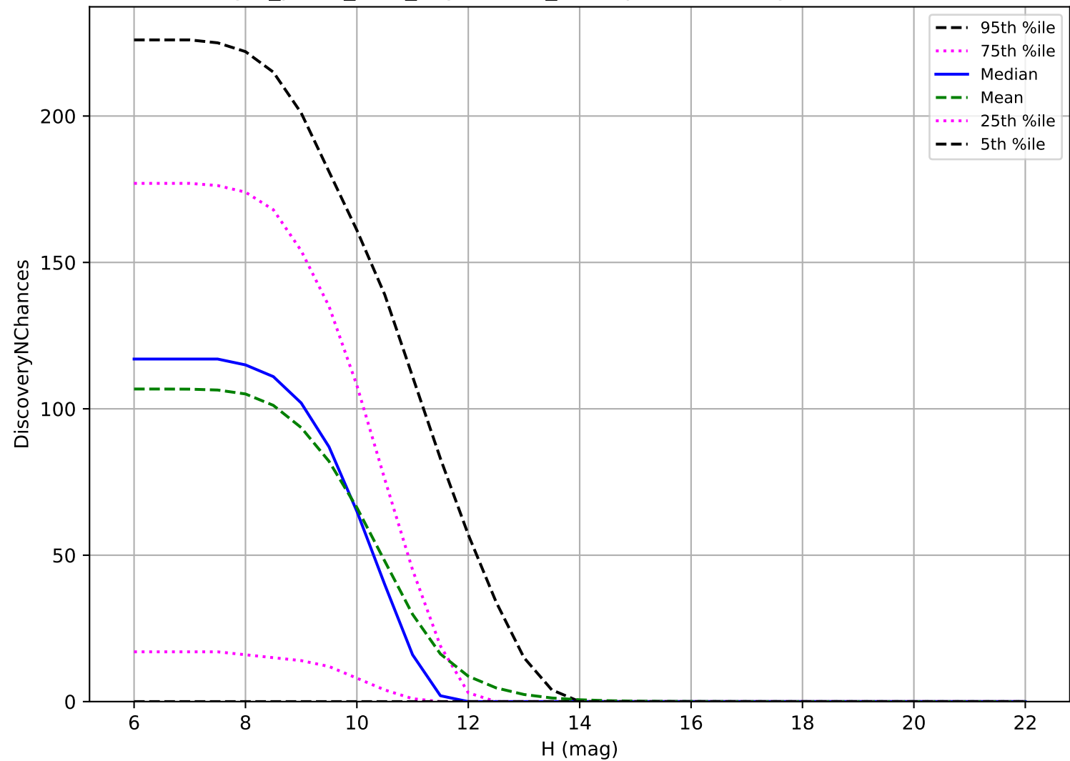
reweight_plane_v3.3_10yrs: OCC_r20 3 pairs in 15 nights detection loss
