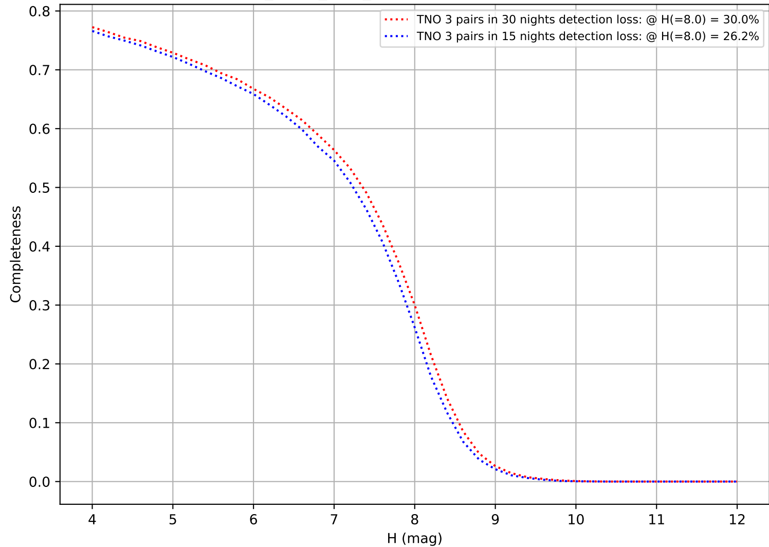
reweight_plane_v3.3_10yrs: DifferentialCompleteness
