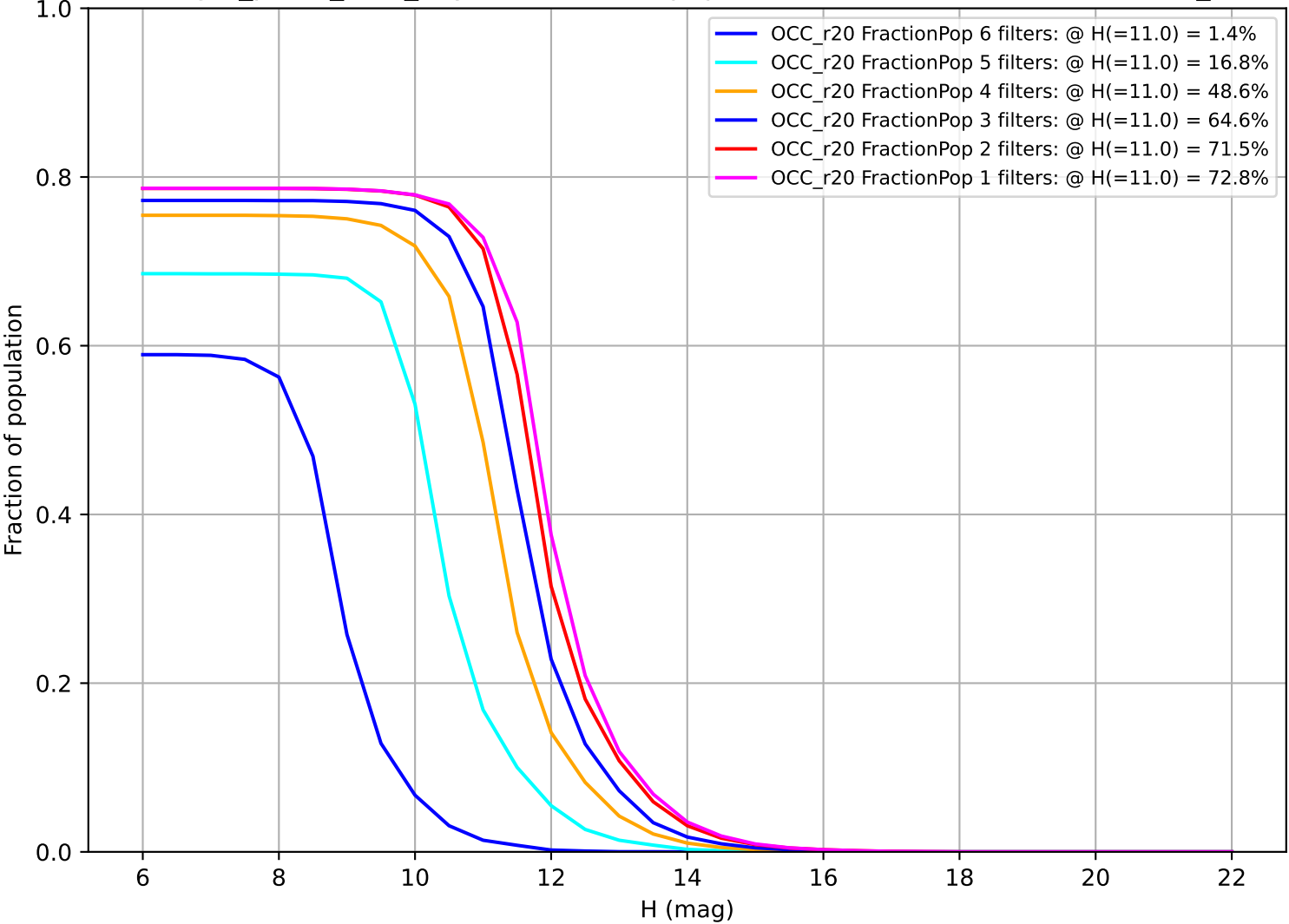
reweight_plane_v3.3_10yrs: Fraction of population with colors in X filters OCC_r20
