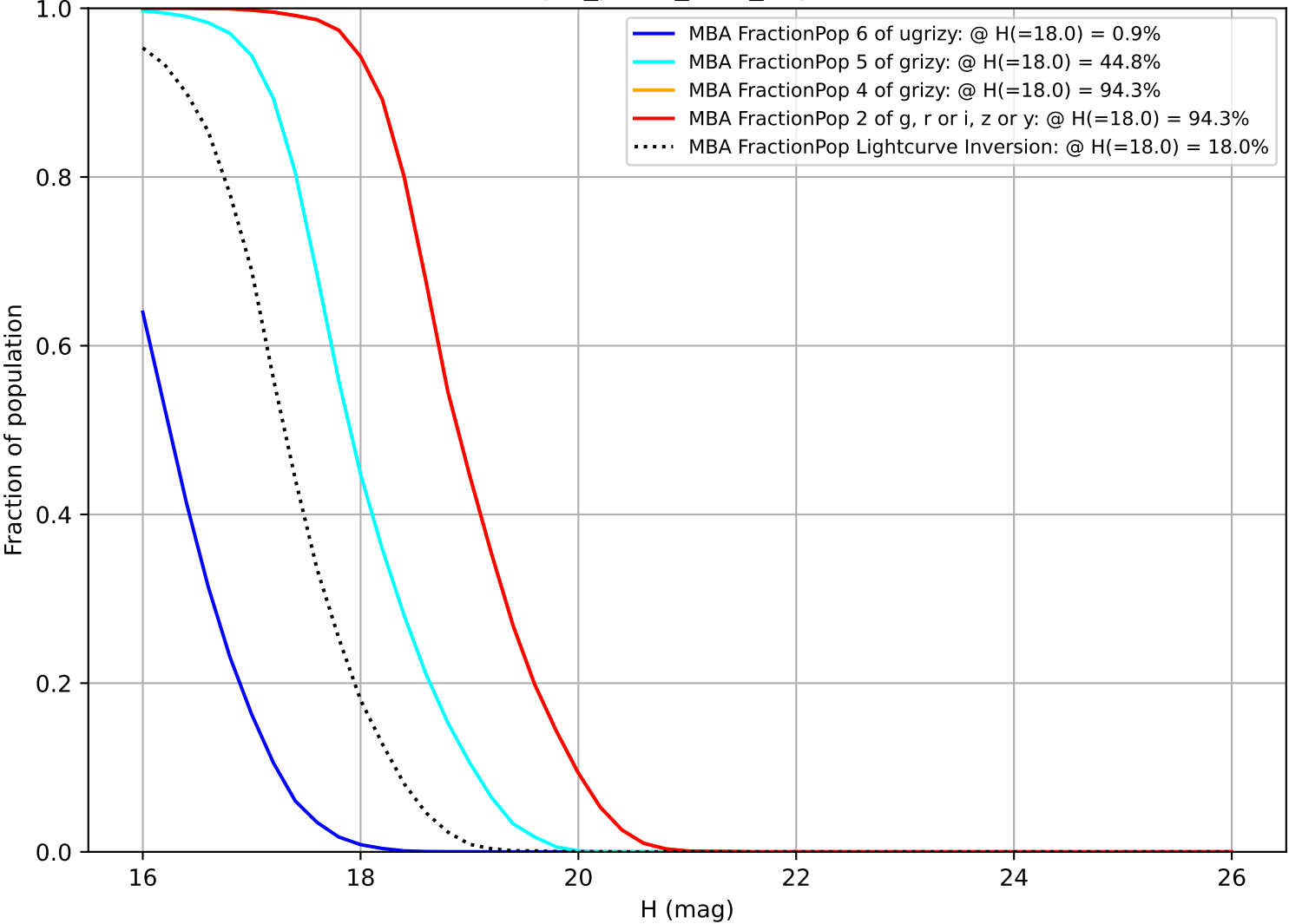
reweight_plane_v3.3_10yrs MBA
