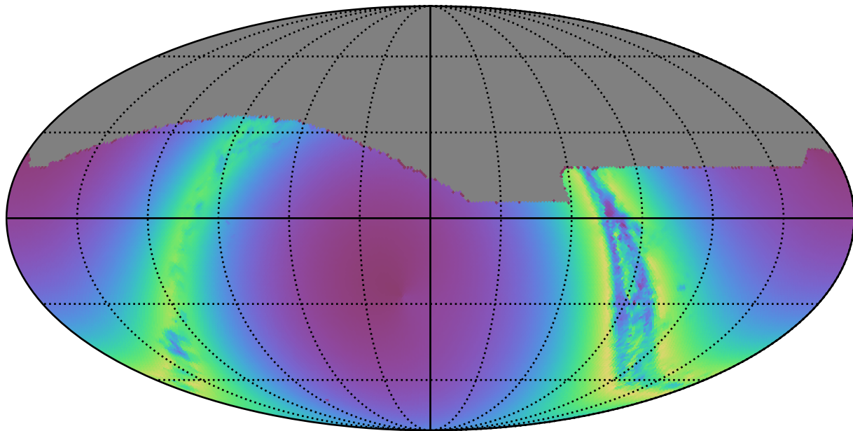
reweight_plane_v3.3_10yrs : young_stars
