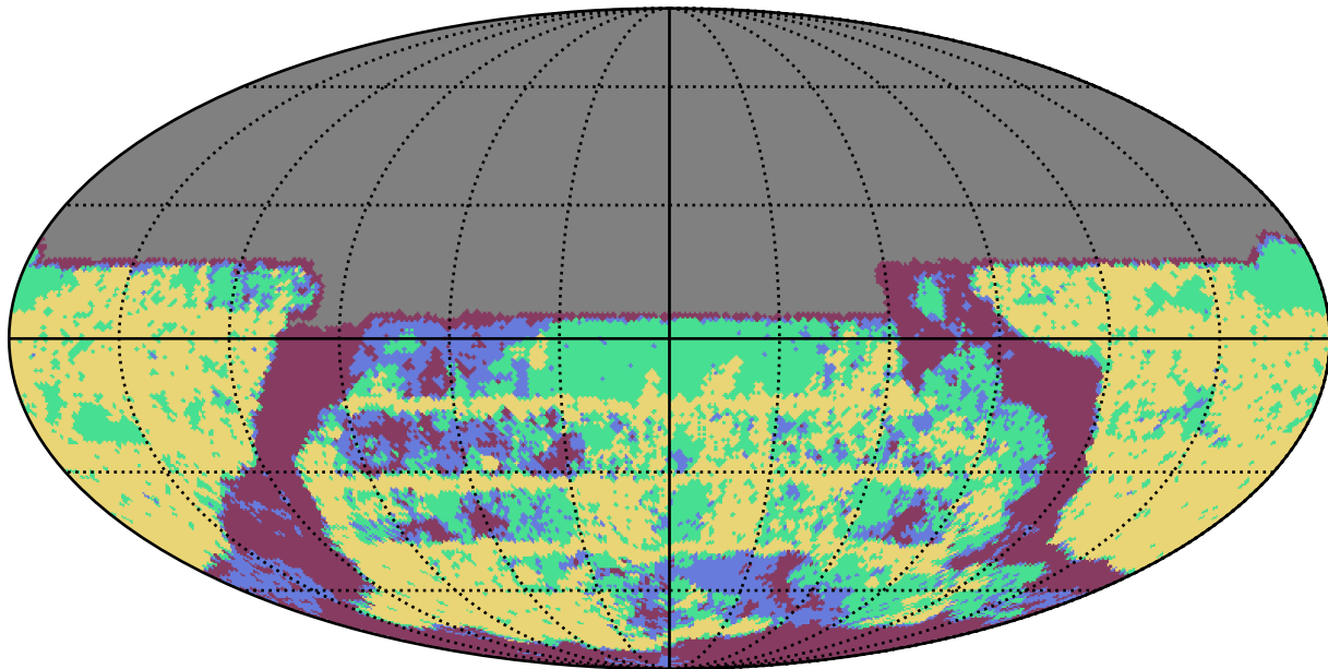
reweight_plane_v3.3_10yrs u band: YearCoverage night
