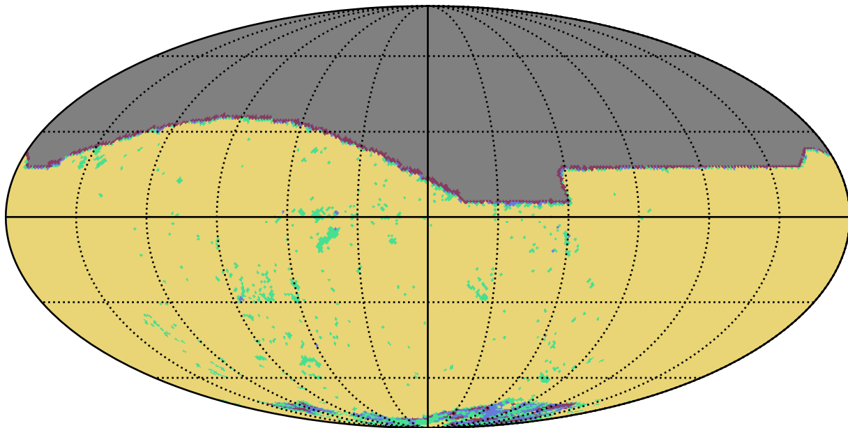
reweight_plane_v3.3_10yrs i band: YearCoverage night
