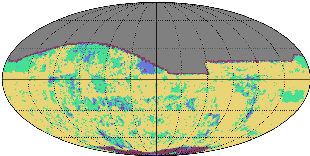
reweight_plane_v3.3_10yrs g band: YearCoverage night
