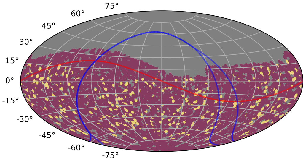
reweight_plane_v3.3_10yrs : TDEsPopMetric_some_color
