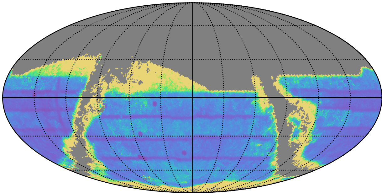
reweight_plane_v3.3_10yrs : TDC_precision
