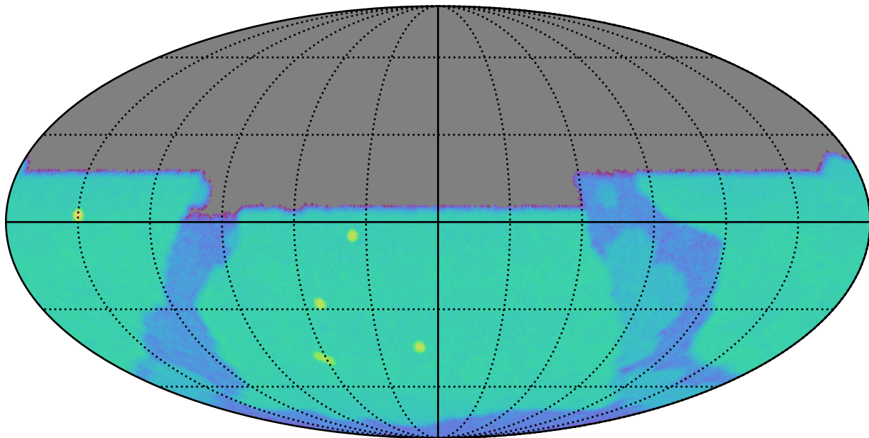
reweight_plane_v3.3_10yrs u: SurfaceBrightLimit
