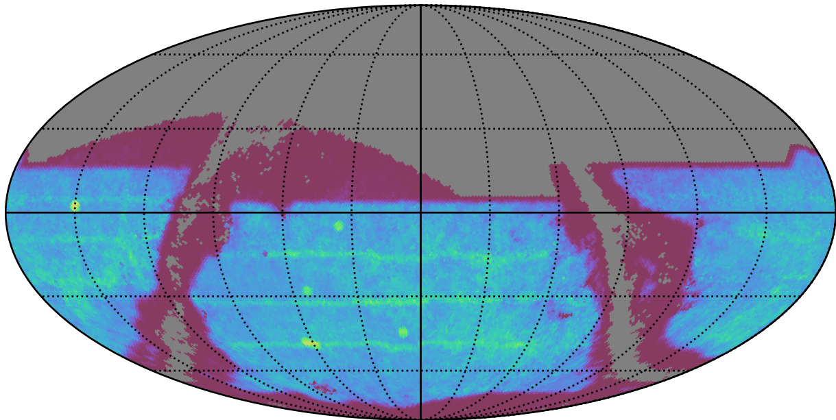
reweight_plane_v3.3_10yrs : SNSLMetric
