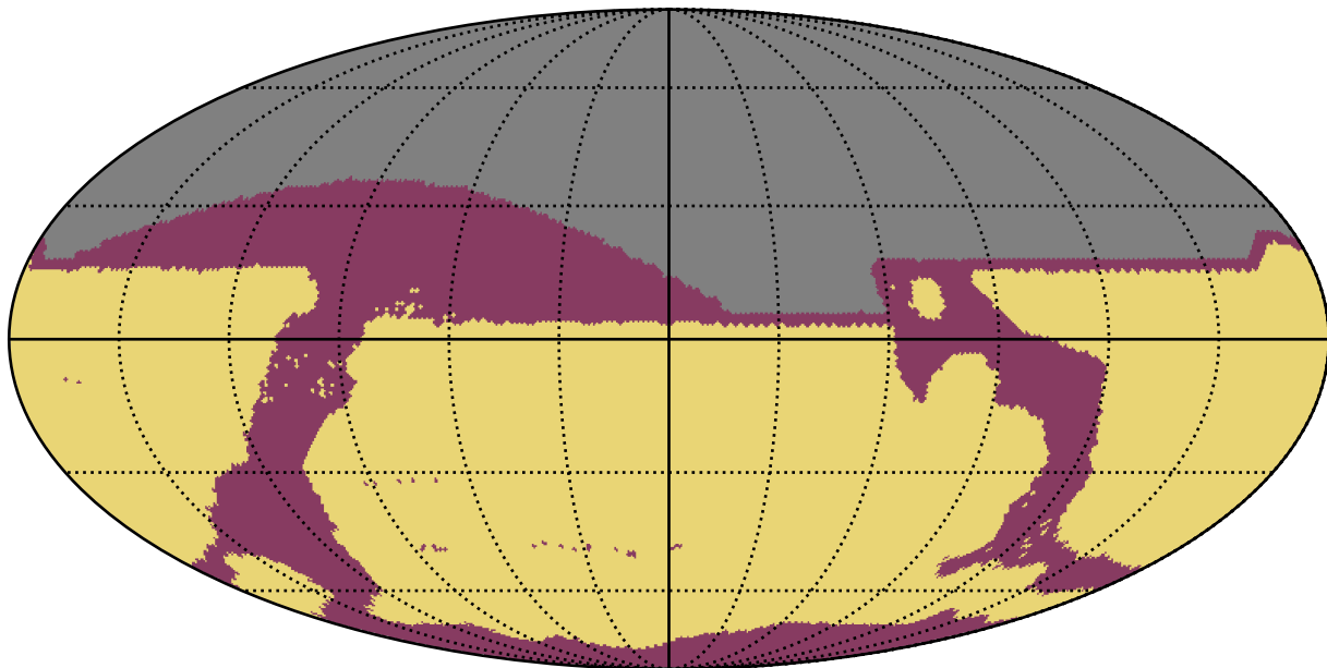
reweight_plane_v3.3_10yrs : RapidRevisits
