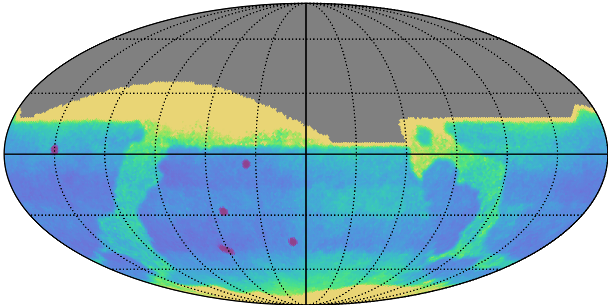
reweight_plane_v3.3_10yrs : Proper Motion Uncert @ 24.0
