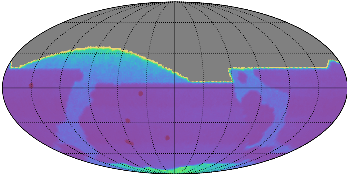
reweight_plane_v3.3_10yrs : Proper Motion Uncert @ 20.5
