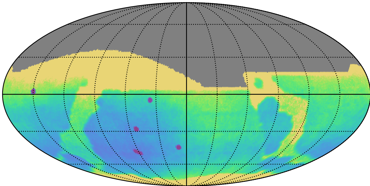
reweight_plane_v3.3_10yrs : Parallax Uncert @ 24.0
