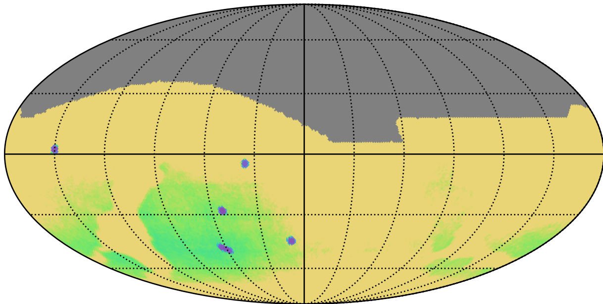
reweight_plane_v3.3_10yrs : Parallax Uncert @ 22.4
