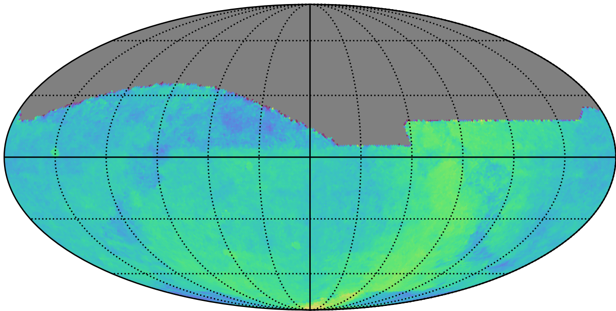
reweight_plane_v3.3_10yrs : Parallax Coverage @ 24.0
