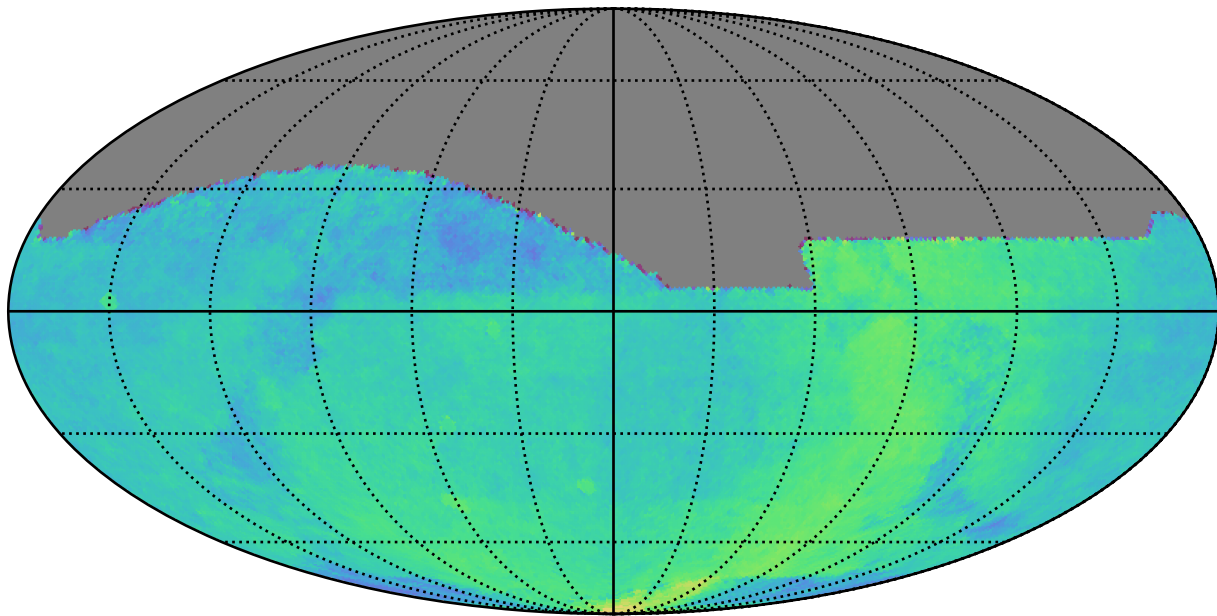
reweight_plane_v3.3_10yrs : Parallax Coverage @ 22.4
