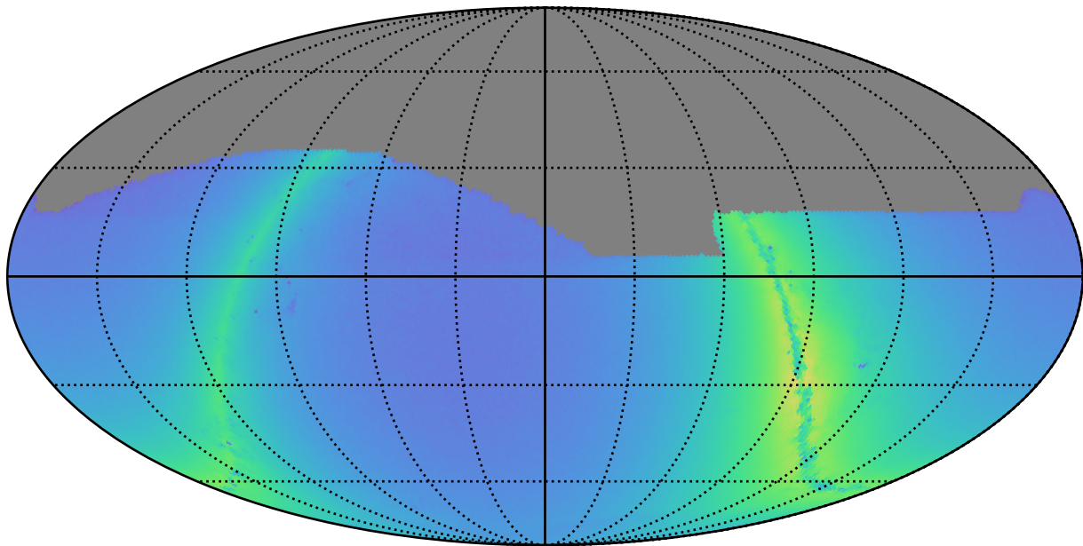
reweight_plane_v3.3_10yrs z: Nstars_no_crowding
