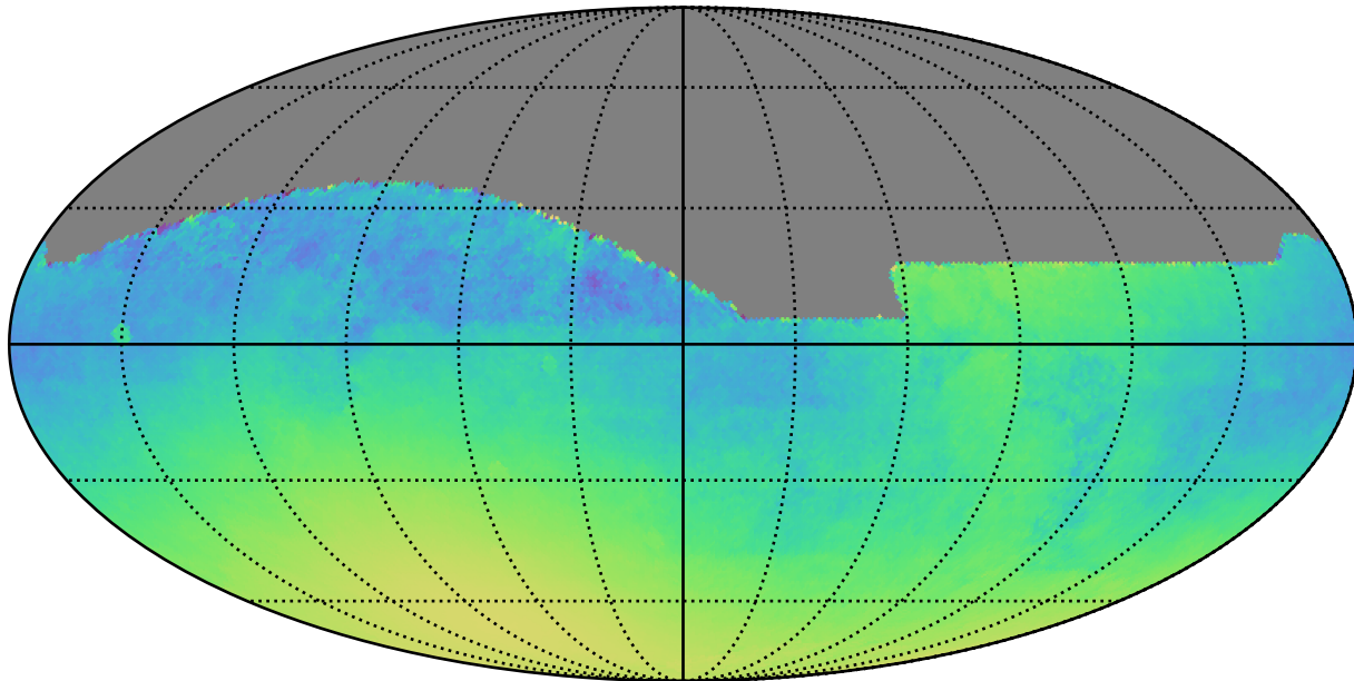
reweight_plane_v3.3_10yrs : Normalized Parallax Uncert @ 24.0
