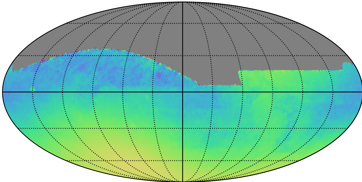
reweight_plane_v3.3_10yrs : Normalized Parallax Uncert @ 22.4
