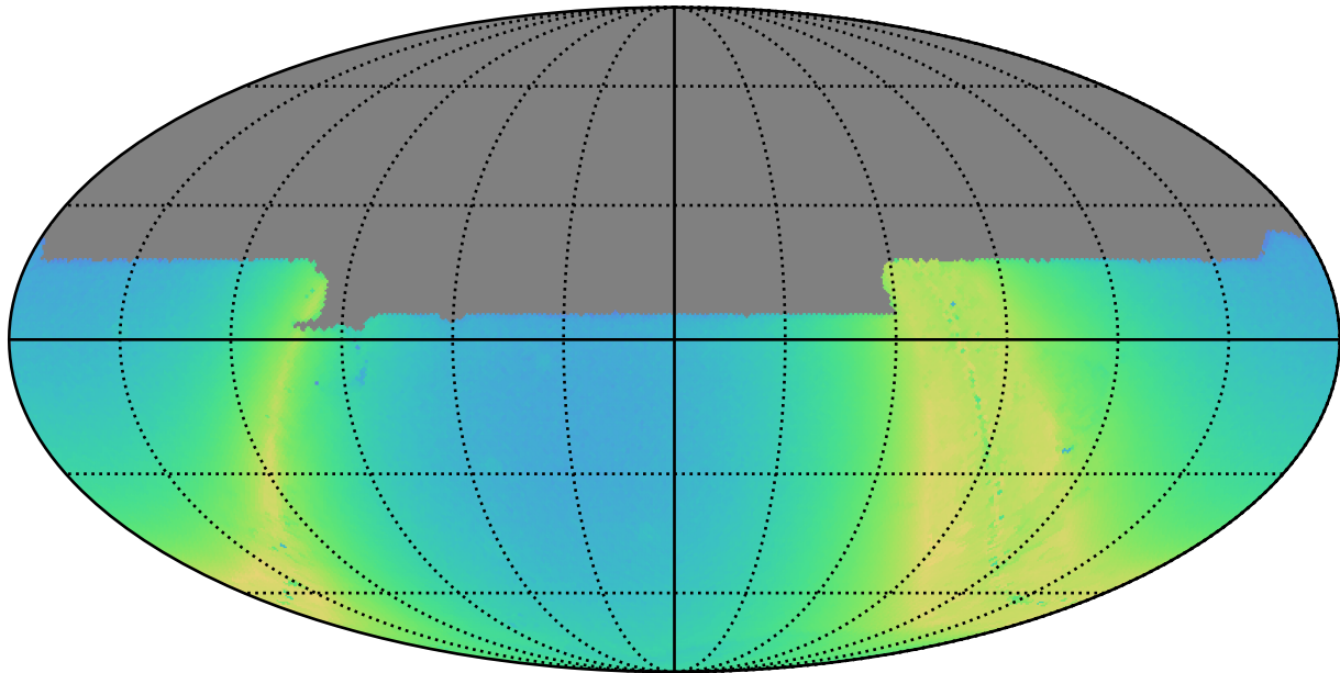
reweight_plane_v3.3_10yrs y: N stars to Precision 0.20
