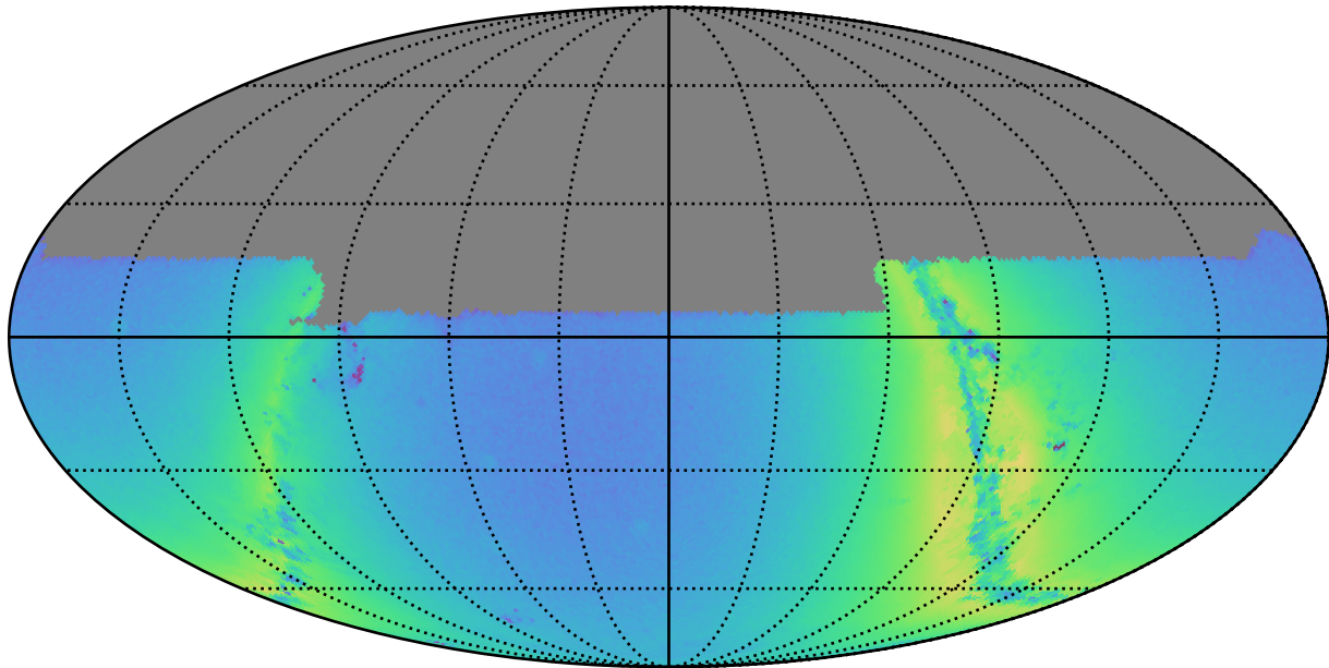
reweight_plane_v3.3_10yrs u: N stars to Precision 0.20
