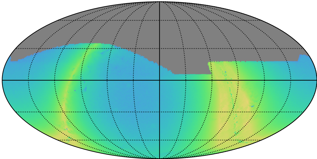
reweight_plane_v3.3_10yrs r: N stars to Precision 0.20
