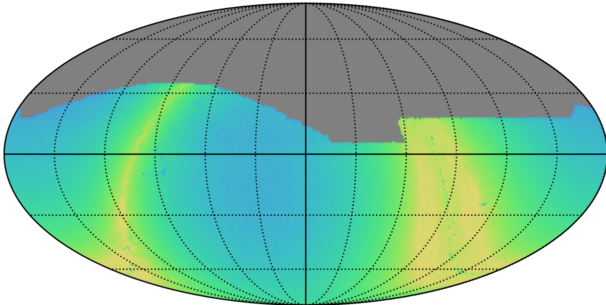
reweight_plane_v3.3_10yrs i: N stars to Precision 0.20
