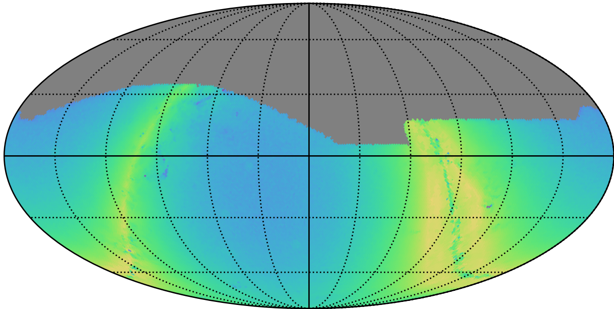
reweight_plane_v3.3_10yrs g: N stars to Precision 0.20
