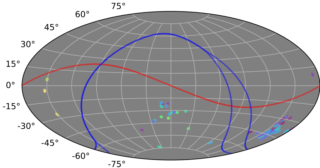
reweight_plane_v3.3_10yrs gi: LVDwarfs
