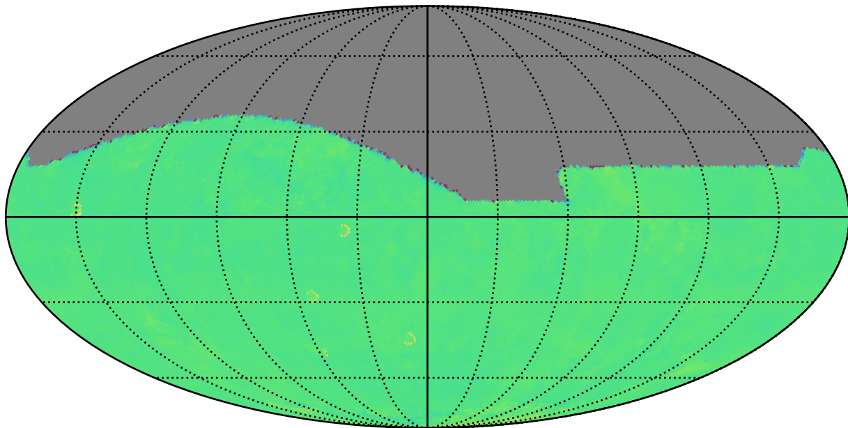
reweight_plane_v3.3_10yrs r: Kuiper rotTelPos
