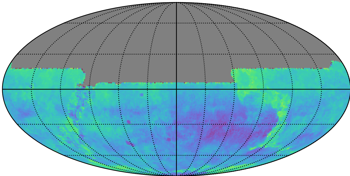
reweight_plane_v3.3_10yrs y: Kuiper rotSkyPos
