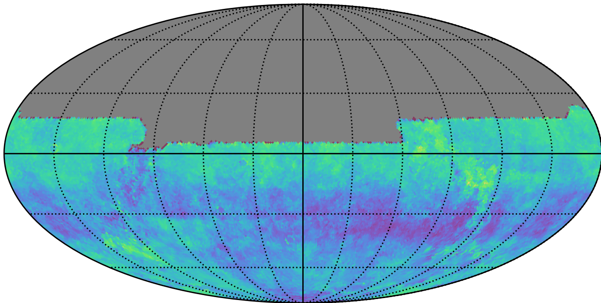
reweight_plane_v3.3_10yrs u: Kuiper rotSkyPos
