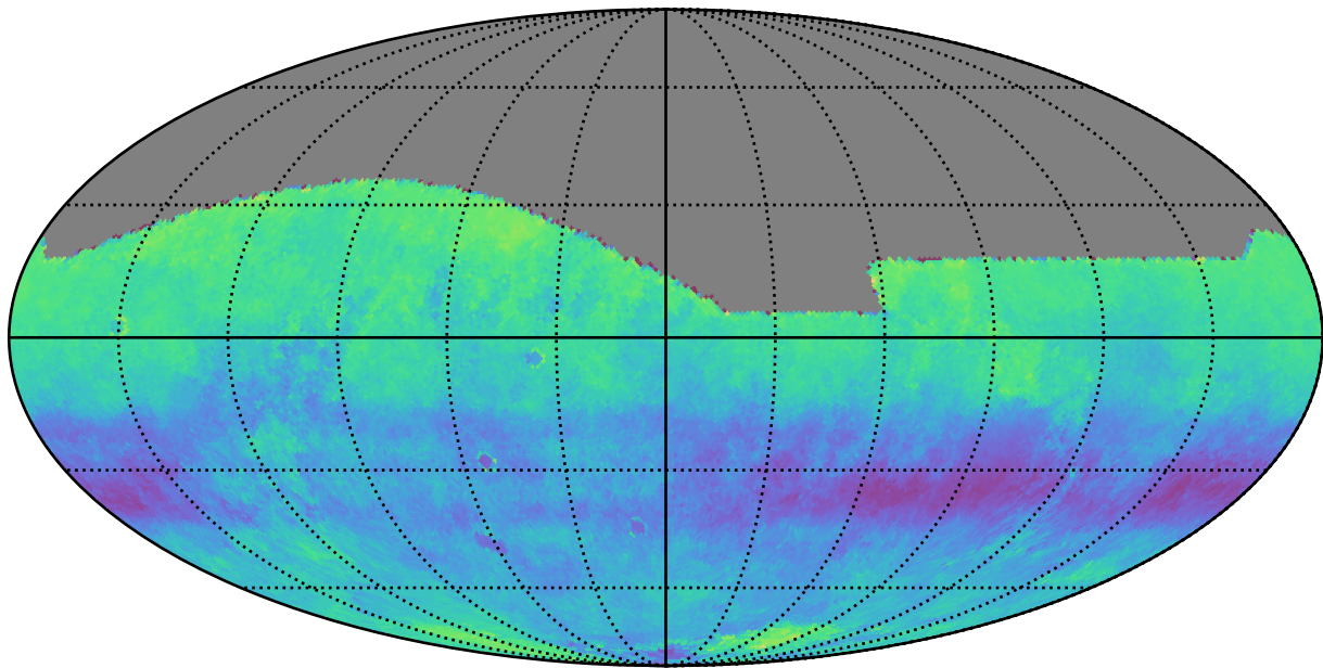
reweight_plane_v3.3_10yrs r: Kuiper rotSkyPos
