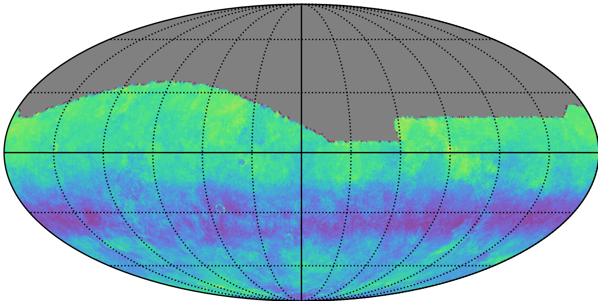
reweight_plane_v3.3_10yrs g: Kuiper rotSkyPos
