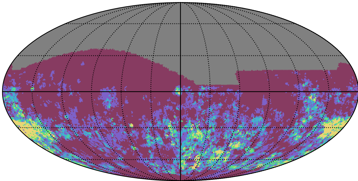
reweight_plane_v3.3_10yrs i band: Gaps_7hr
