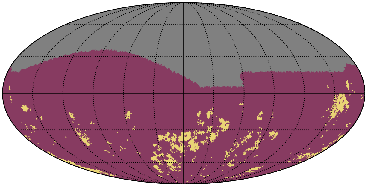
reweight_plane_v3.3_10yrs g band: Gaps_7hr
