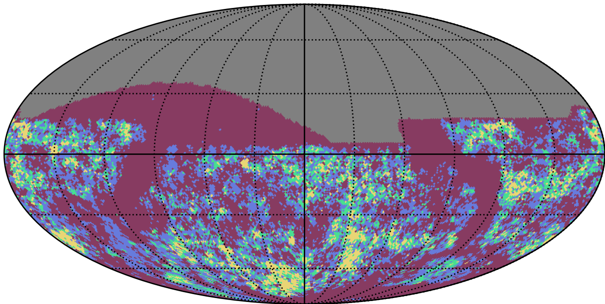
reweight_plane_v3.3_10yrs z band: Gaps_3hr
