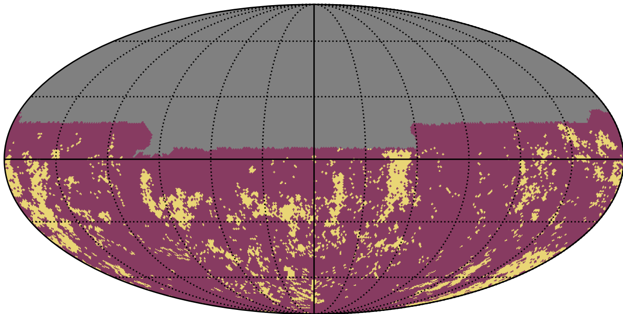
reweight_plane_v3.3_10yrs u band: Gaps_3hr
