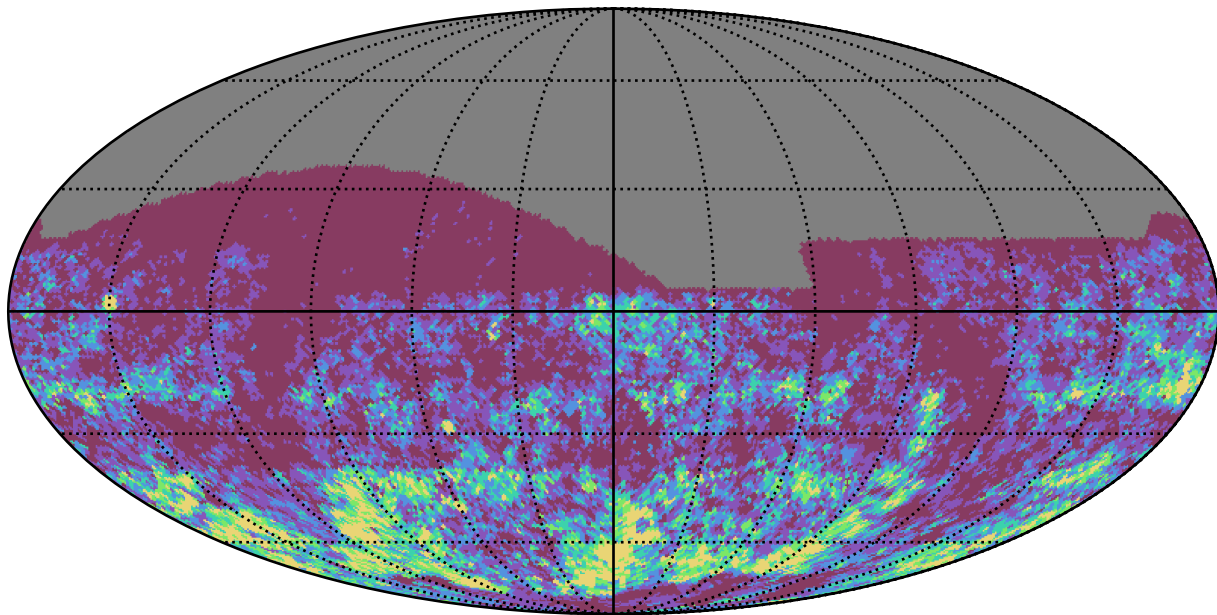
reweight_plane_v3.3_10yrs r band: Gaps_3hr
