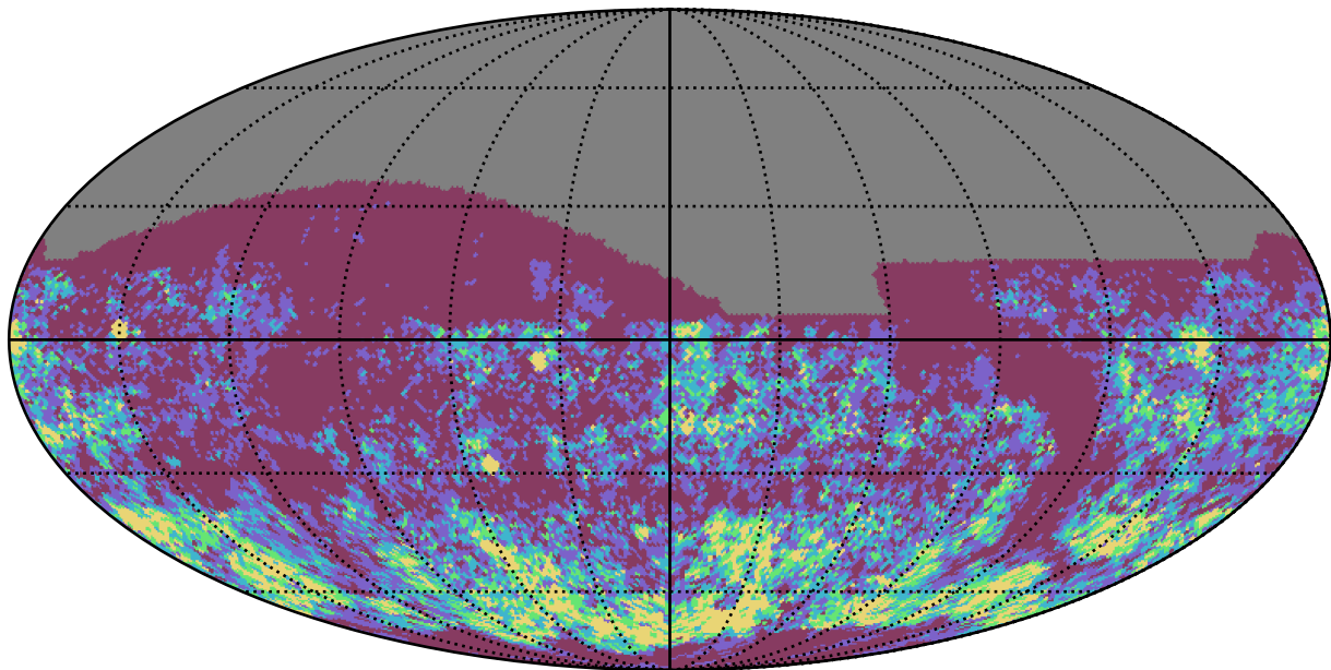
reweight_plane_v3.3_10yrs i band: Gaps_3hr
