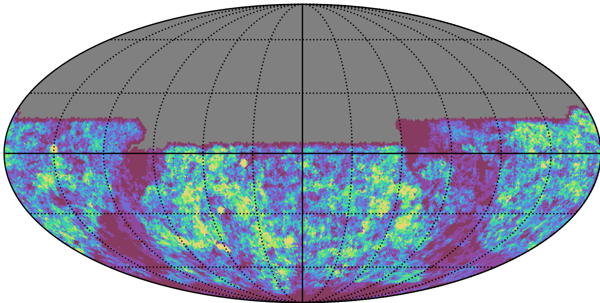
reweight_plane_v3.3_10yrs u band: Gaps_24hr
