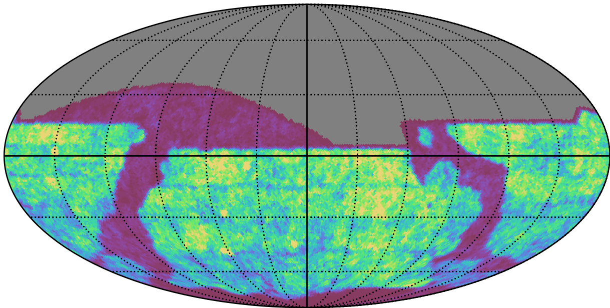
reweight_plane_v3.3_10yrs r band: Gaps_24hr
